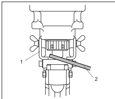
► 1. Stripper 2. Workpiece
